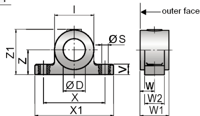
Mounting brackets*
