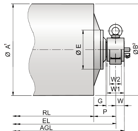
Idler Pulley 3 UT630M / UT630H
